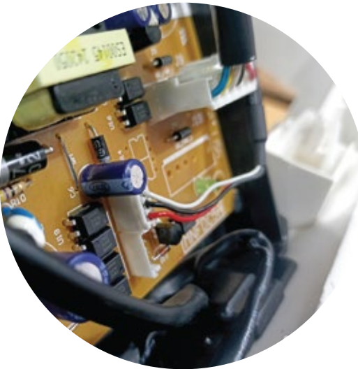
Indoor unit Board
